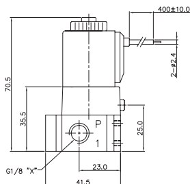
YSV310-DP-SD2-*** Normally Closed
