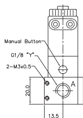
YSV320-DP-SG2-*** Normally Open
