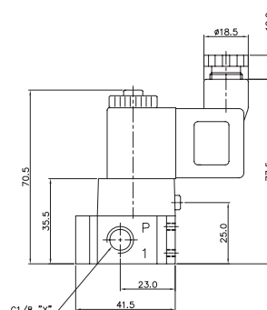
YSV310-DP-SC2-CN2-*** Normally Closed
