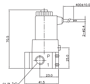
YSV310-DP-SG2-*** Normally Closed
