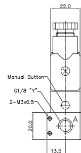
YSV320-DP-SC2-CN2-*** Normally Open
