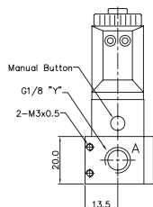
YSV320-DP-SD2-*** Normally Open
